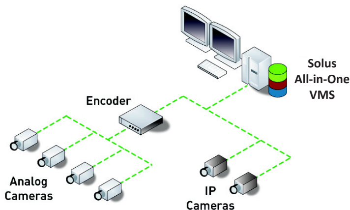
Typical All-in-One VMS Configuration
